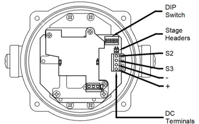
Fig. 4 S110 DC Terminals
