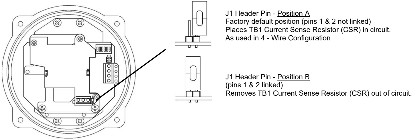
Figure 12: J1 Header pin positions – Current Sense Resistor (CSR)
