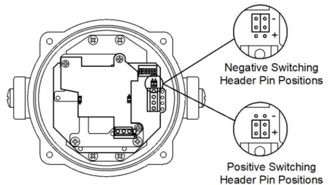
Fig. 5 Stage Switching Polarity
