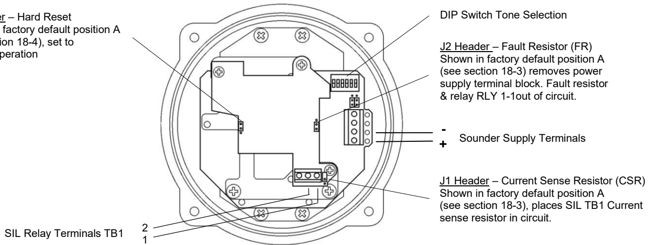
Figure 9 – Terminals and header pins for sounder
