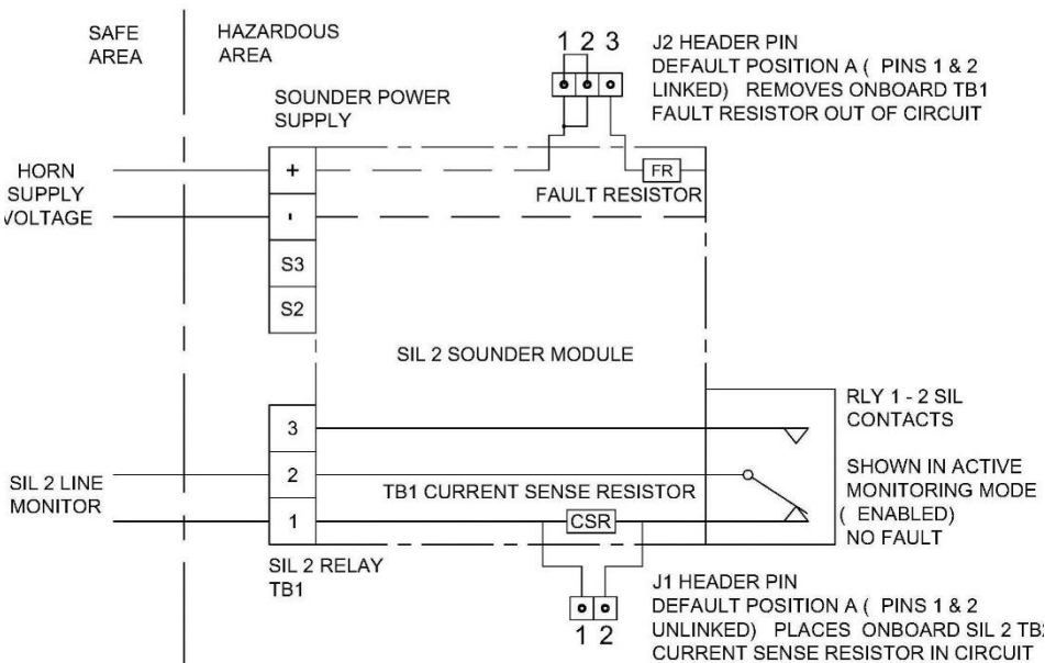
Figure 10 - Schematic of SIL 2 system wiring for fault detection in standby and active mode – 4 wire installation.
