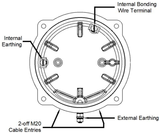
Fig. 3 Internal View of Cover
