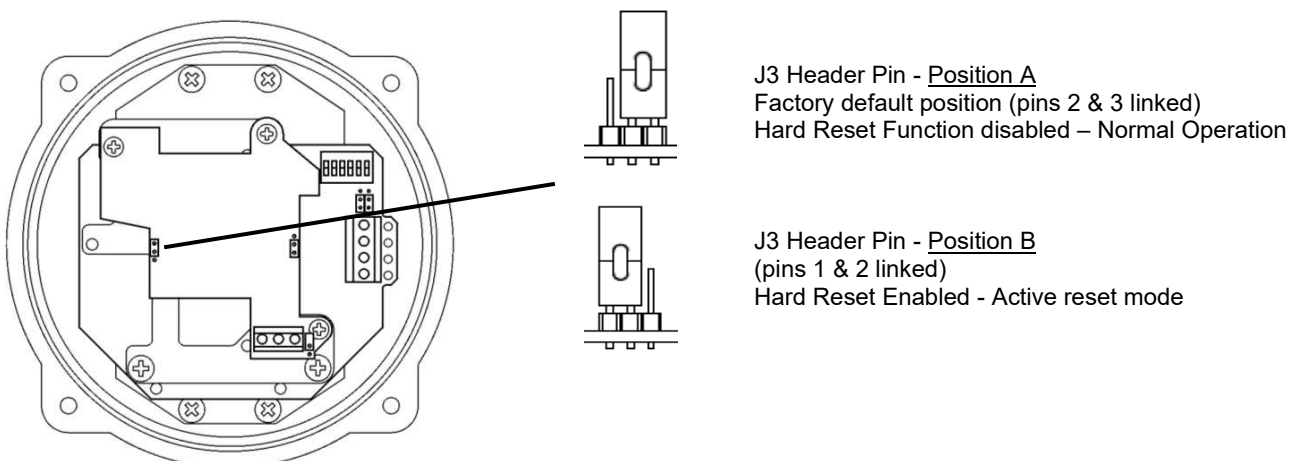
Figure 14: J3 Header pin positions – Hard Reset Function
