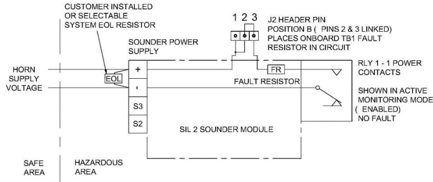
Figure 11 - Schematic of SIL 2 system wiring for fault detection in standby mode only – 2 wire installation
