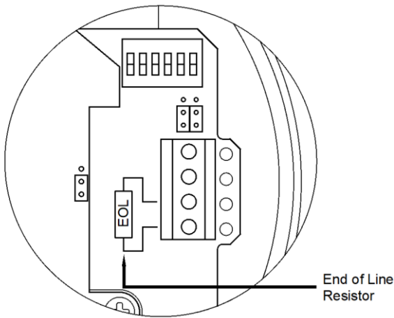
Fig. 6 End of Line Resistor Placement
