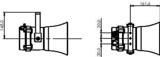
Fig. 1 Fixing Location for S110 Sounder
