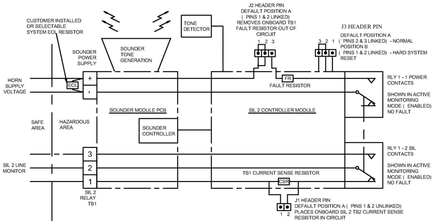
Figure 8 - The SIL 2 Module monitors the Sounder and interfaces to the customer plant.
