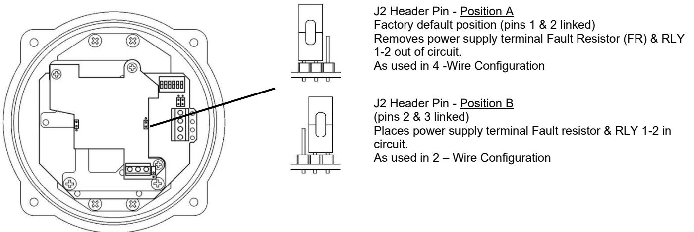
Figure 13: J2 Header pin positions – Fault Resistor (FR)
