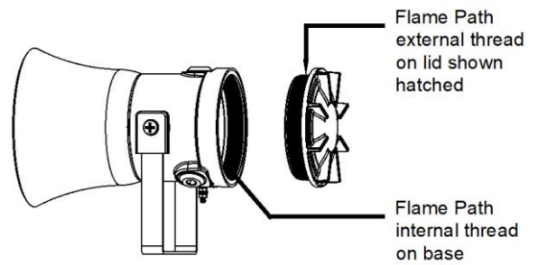
Figure 1: Flame Path
