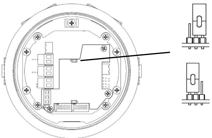
Figure 18: J3 Header pin positions – Hard Reset Function
