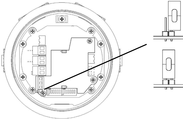
Figure 16: J1 Header pin positions – Current Sense Resistor (CSR)
