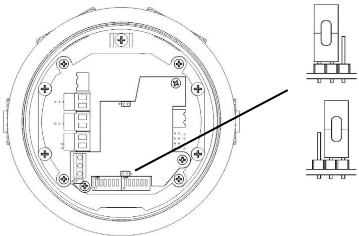
Figure 17: J2 Header pin positions – Fault Resistor (FR)
