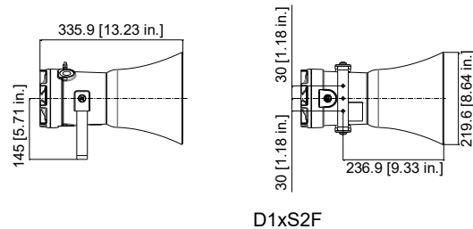
Fig 1: Mounting Locations
