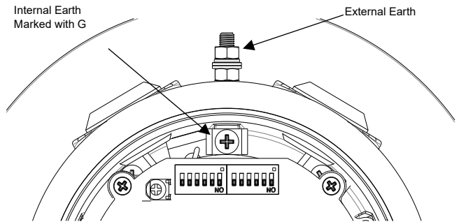
Fig. 4 Earth Locations
